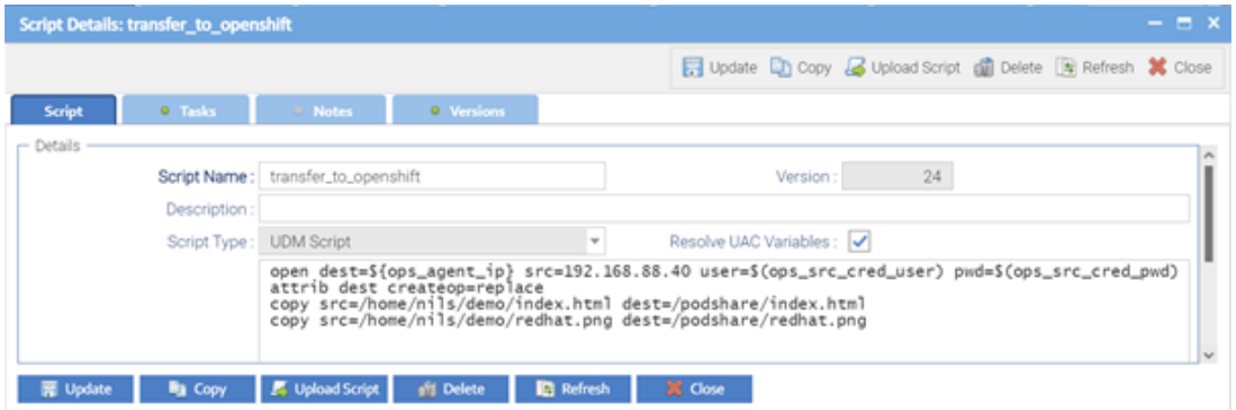
Universal Controller File Transfer Task script
