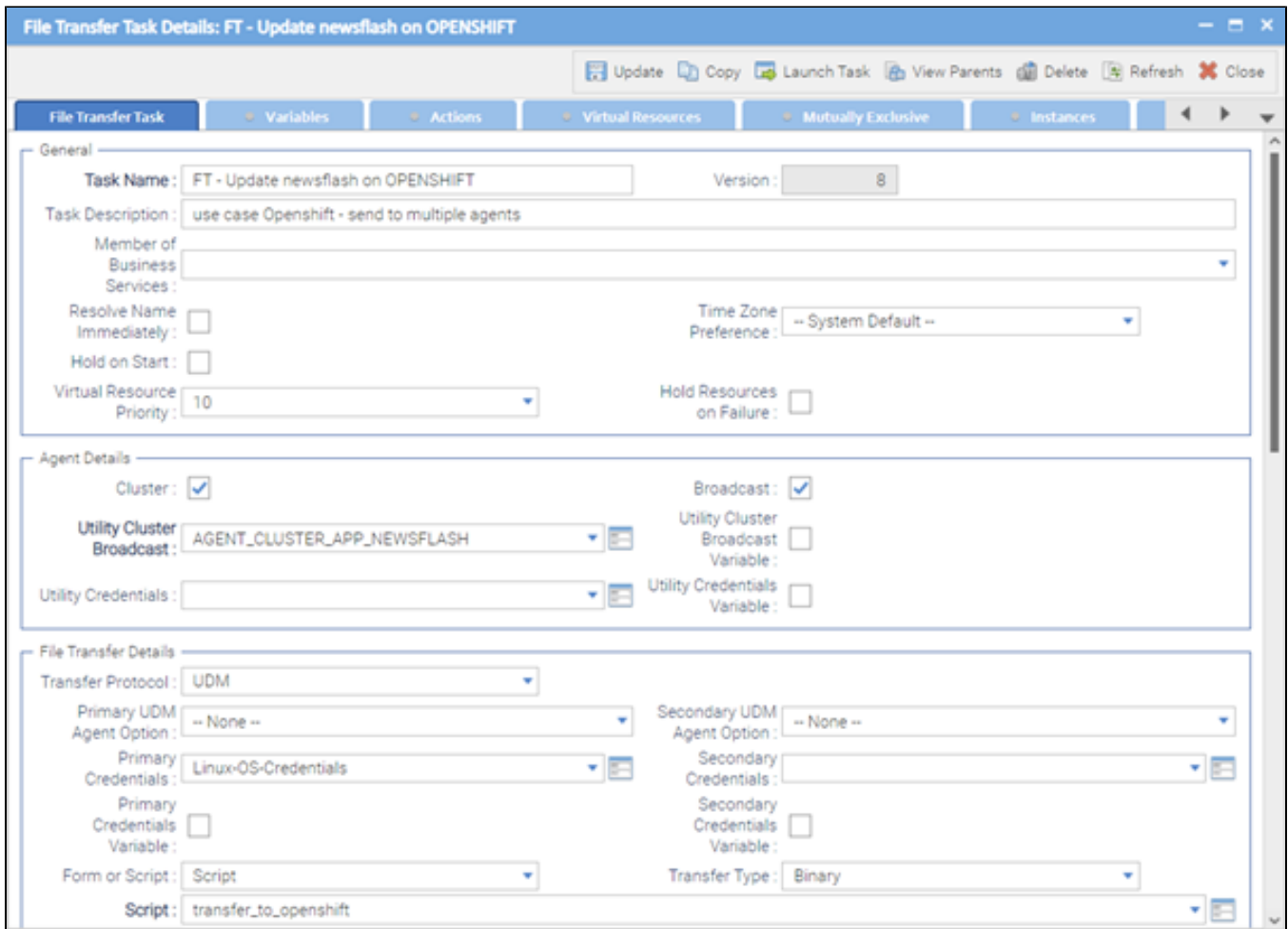
Universal Controller File Transfer Task
